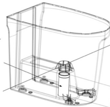
Straight pipe installation
