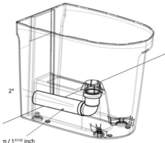
90° pipe installation
