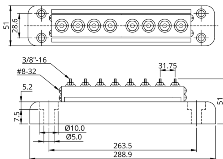
Busbar 600 A with 8 high current terminals and 8 low current screw terminals, without cover
